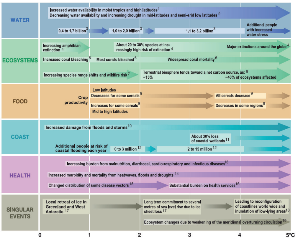
Figure 4: Examples of global impacts projected for changes in climate (and sea level and atmospheric carbon dioxide where relevant) associated with different amounts of increase in global average surface temperature in the 21 st century. This is a selection of some estimates available for inclusion in IPCC (2007b). All entries are taken from published studies that are referenced in chapters of IPCC (2007b). Edges of boxes and placing of text indicate the range of temperature change to which the impacts relate. Arrows between boxes indicate increasing levels of impacts between estimations. Other arrows indicate trends in impacts. All entries for water stress and flooding represent the additional impacts of climate change relative to the conditions projected across the range of projected scenarios. Adaptation to climate change is not included in these estimations. For extinctions, ‘major’ means ~40 to ~70% of assessed species. Source: IPCC (2007b), Table TS.3, p.66.
